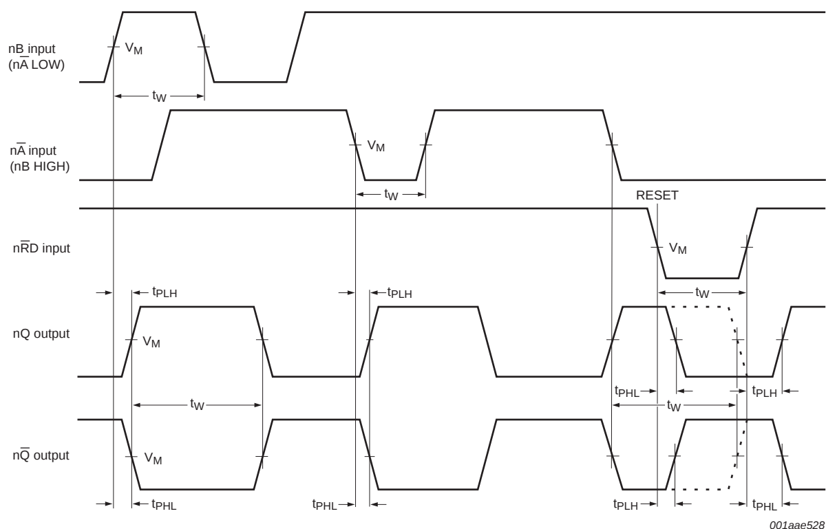
Fig 7. Propagation delays from inputs ( \bar{nA} , nB , \bar{nRD} ) to outputs ( nQ , \bar{nQ} )
